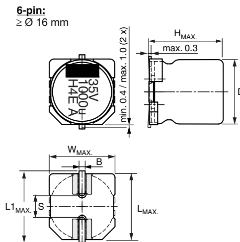
Fig. 1 - Dimensional outline
